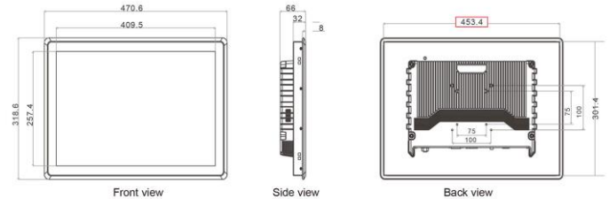
19" Widescreen Touch Monitor
