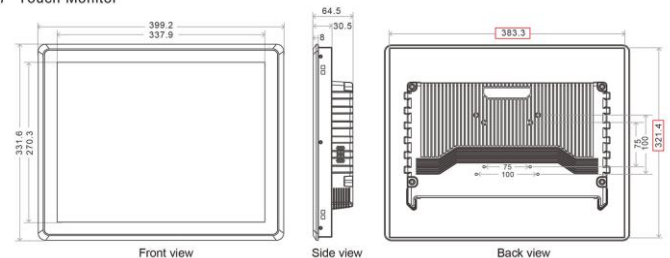
17" Touch Monitor
