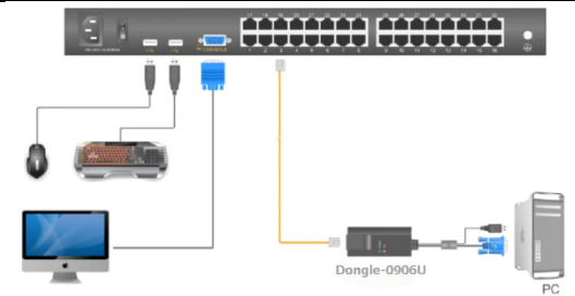
Connection Diagram
